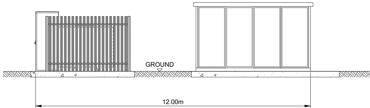
ELEVATION 'A'
